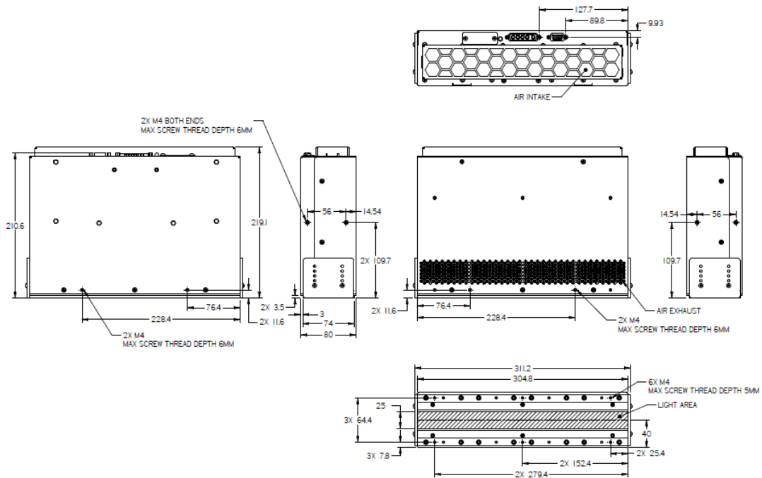
Figure 3 AC9300 UV LED Head Mechanical Drawings
